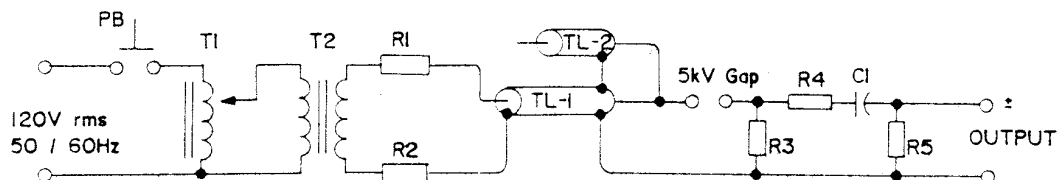
Figure B.1—Typical Oscillatory SWC Test Circuit
