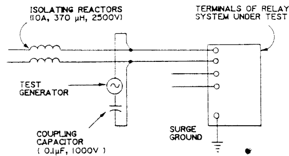
Figure 4—Application of Transverse Mode Tests and Typical Component Values
