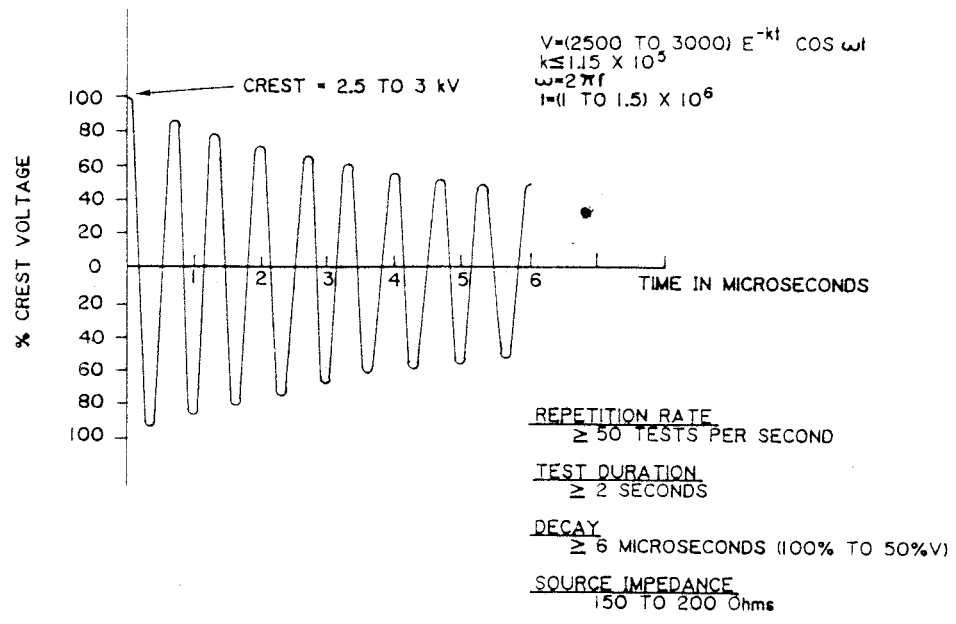
Figure C.1—Typical Oscillatory SWC Test Wave (Open Circuit)
