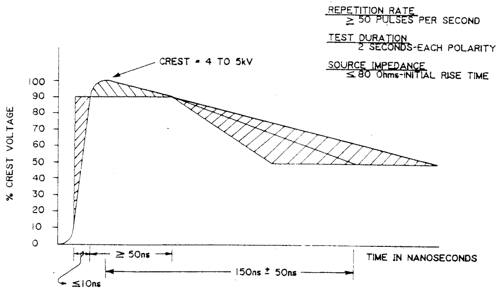
Figure C.2—Typical Fast Transient SWC Test Wave (Open Circuit)
