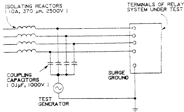
Figure 3—Application of Common Mode Tests and Typical Component Values
