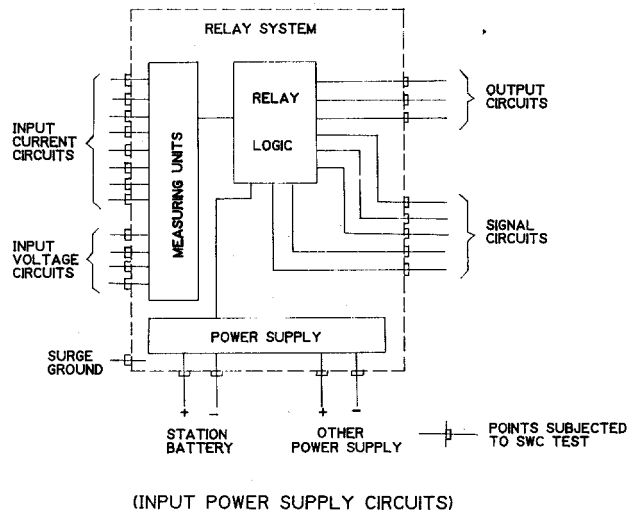
Figure 2—General Makeup of a Relay System without Communications Interface Showing Points to Be Subjected to SWC Tests
