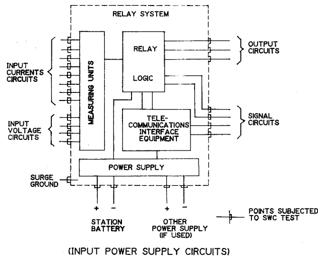
Figure 1—General Makeup of a Relay System with Communications Interface Showing Points to Be Subjected to SWC Tests
